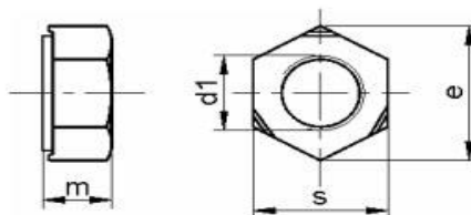
Hexagon Weld Nuts
